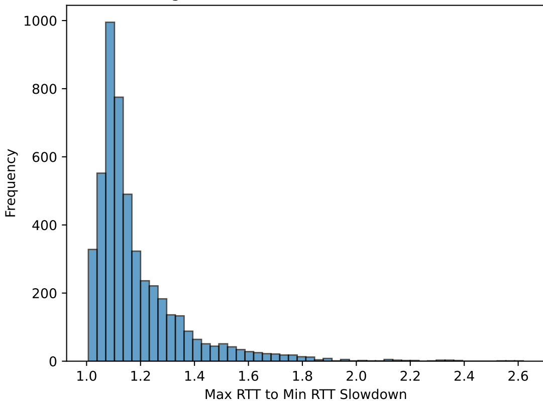
Histogram of Max RTT to Min RTT Slowdown
